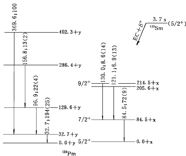
Fig. 1. Proposed decay scheme of ^{133}\text{Sm} .
